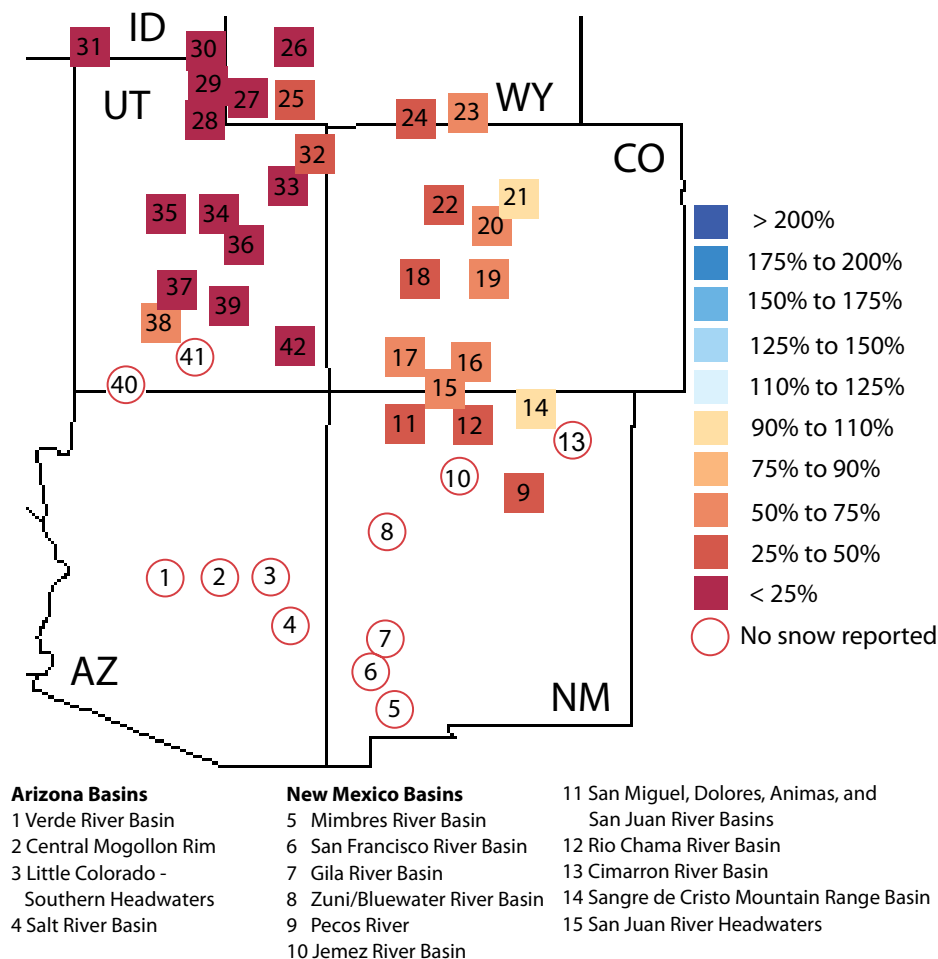
Figure 8. Average snow water content (SWC) in percent of average for available monitoring sites as of May 17, 2007.
