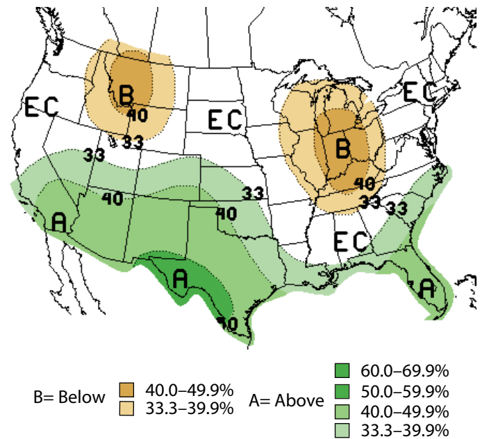
Figure 17a. Long-lead U.S. precipitation forecast for February–April 2007 (issued January 2007).
