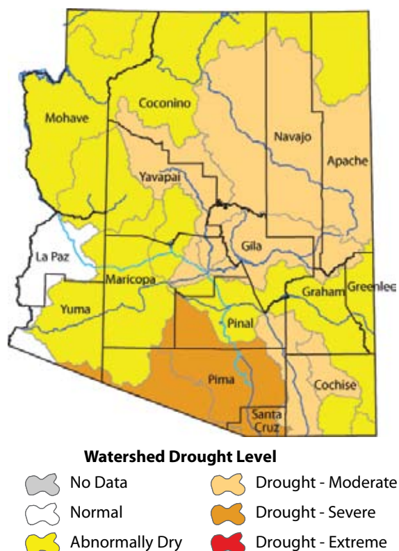
Figure 4b. Arizona long-term drought status for April 2007.
