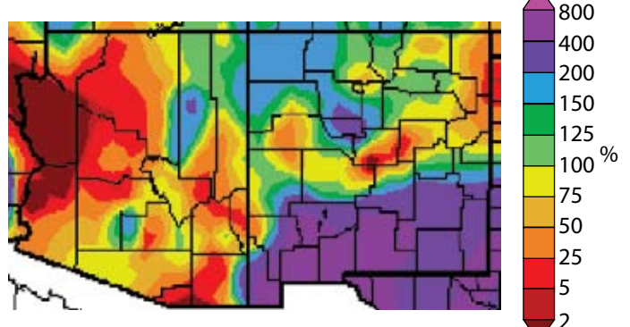
Figure 2d. Previous 30 days (April 17–May 16, 2007) percent of average precipitation (data collection locations only).
