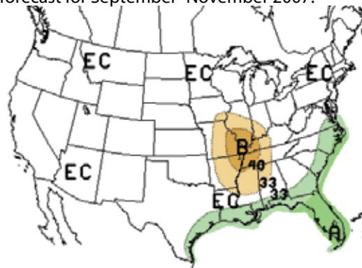
Figure 11d. Long-lead national precipitation forecast for September–November 2007.
