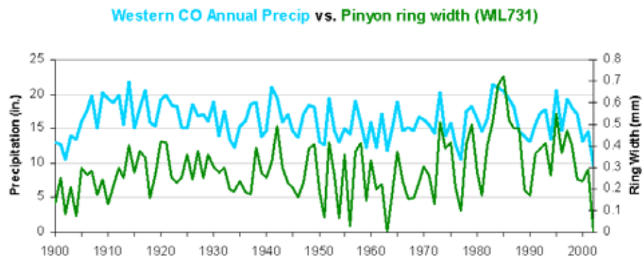
Figure 2: The growth of a pinyon pine sampled in western Colorado near the Delta explains about 70 percent of the variability in annual precipitation for western Colorado. The strong moisture signal recorded in the trees is the basis for robust tree-ring reconstructions of streamflow in the region.
