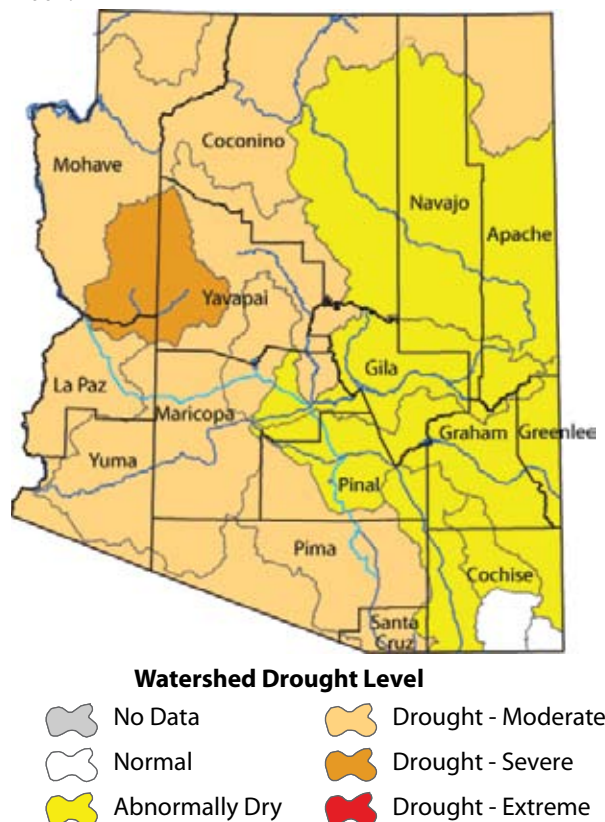
Figure 4a. Arizona short-term drought status for April 2007.
