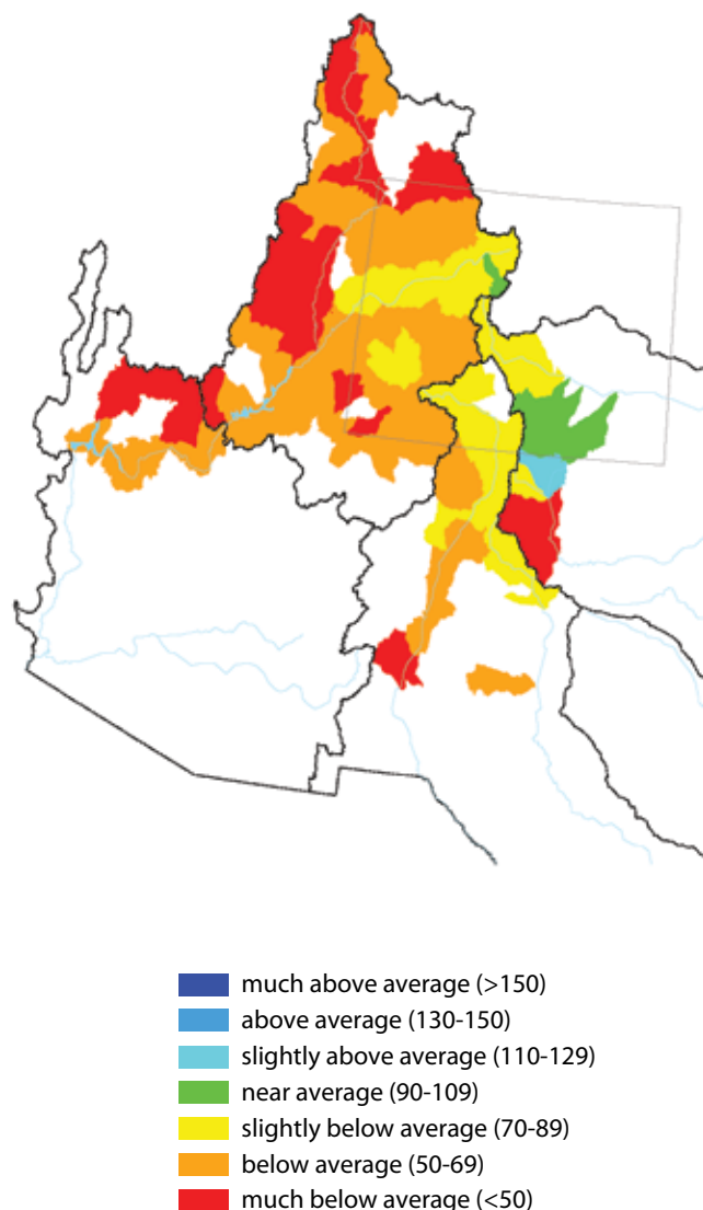
Figure 13. Spring and summer streamflow forecast as of May 1, 2007 (percent of average).
