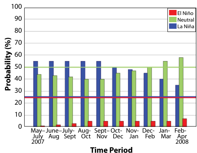
Figure 15b. IRI probabilistic ENSO forecast for El Niño 3.4 monitoring region (released May 17, 2007). Colored lines represent average historical probability of El Niño, La Niña, and neutral.
