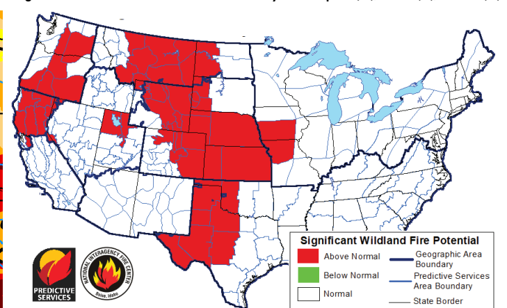
Figure 6: NIFC Significant Wildland Fire Potential Outlook - July 2022
