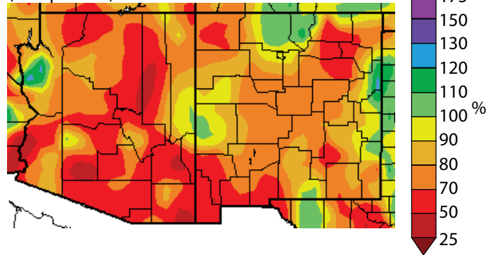
Figure 2b. Water year '08–'09 (through September 16, 2009) percent of average precipitation (data collection locations only).
