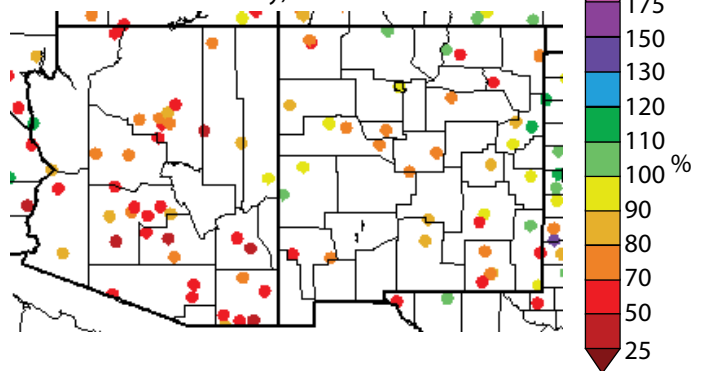
Figure 2c. Previous 30 days (August 18–September 16, 2009) percent of average precipitation (interpolated).
