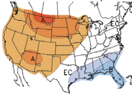
Figure 9d. Long-lead national temperature forecast for January–March 2010.
