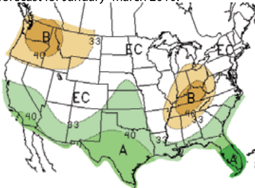
Figure 10d. Long-lead national precipitation forecast for January–March 2010.
