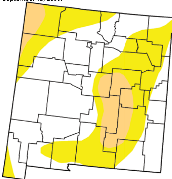
Figure 5a. New Mexico drought map based on data through September 15, 2009.
