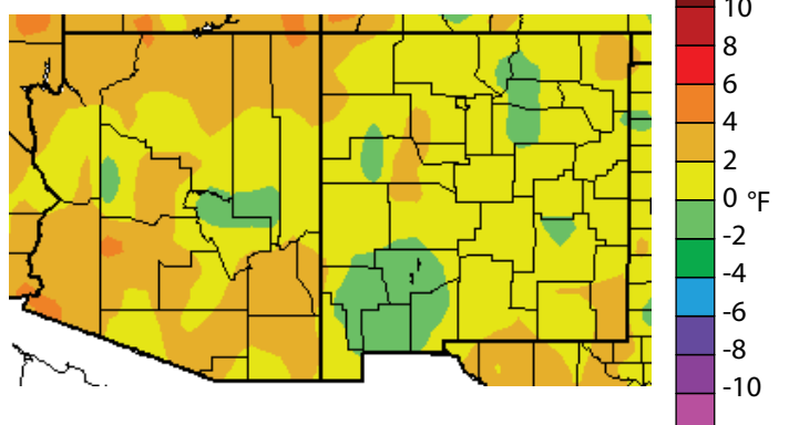
Figure 1d. Previous 30 days (August 18–September 16, 2009) departure from average temperature (data collection locations only).
