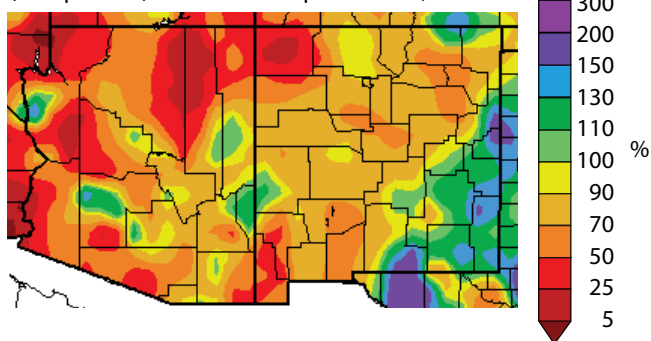
Figure 8c. Percent of average precipitation (interpolated) for June 15–September 12, 2009.
