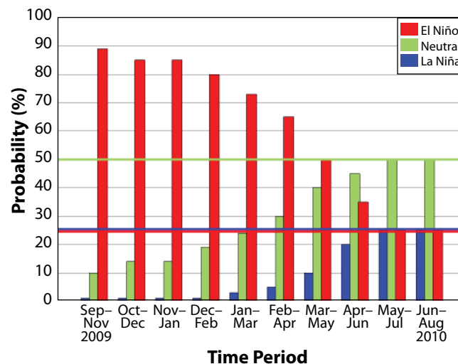
Figure 12b. IRI probabilistic ENSO forecast for El Niño 3.4 monitoring region (released September 17, 2009). Colored lines represent average historical probability of El Niño, La Niña, and neutral.
