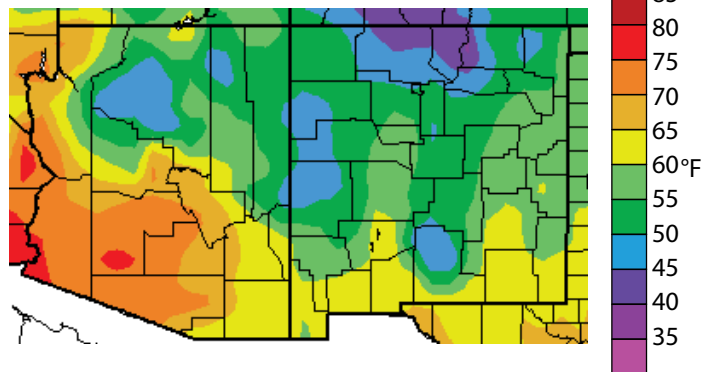
Figure 1b. Water year '08–'09 (through September 16, 2009) departure from average temperature.
