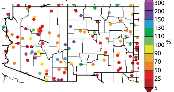
Figure 2d. Previous 30 days (August 18–September 16, 2009) percent of average precipitation (data collection locations only).
