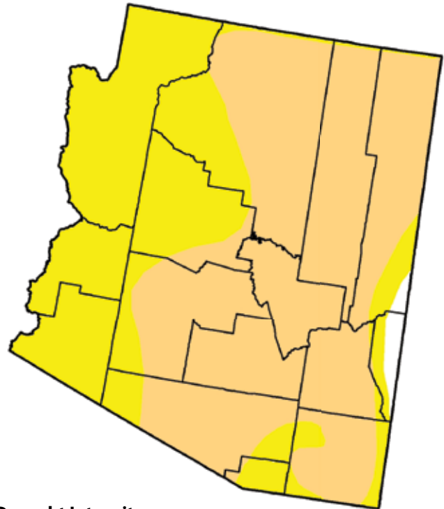
Figure 4a. Arizona drought map based on data through September 15, 2009.
