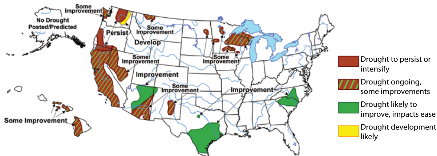
Figure 11. Seasonal drought outlook through December 2009 (released September 17, 2009).
