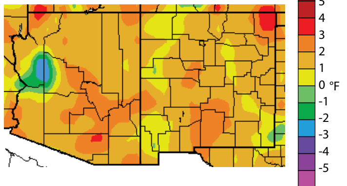
Figure 1c. Previous 30 days (August 18–September 16, 2009) departure from average temperature (interpolated).
