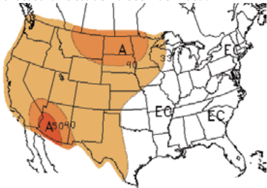
Figure 9c. Long-lead national temperature forecast for December 2009–February 2010.
