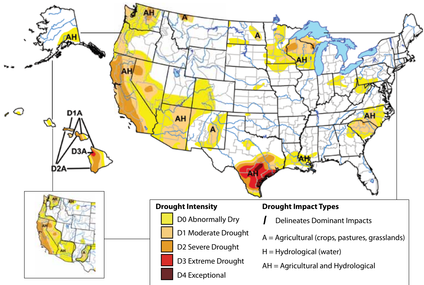
Figure 3. Drought Monitor released September 17, 2009 (full size), and August 20, 2009 (inset, lower left).
