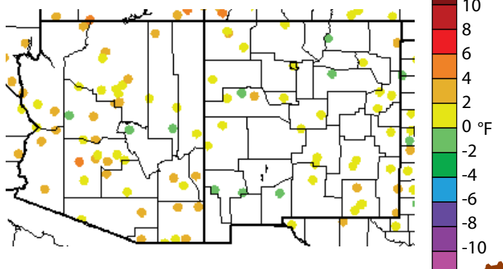
Figure 1d. Previous 30 days (August 18–September 16, 2009) departure from average temperature (data collection locations only).
