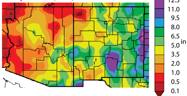
Figure 8b. Departure from average precipitation in inches (June 15–September 12, 2009).
