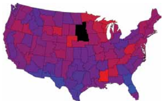
Figure 14c. RPSS for December 2009–February 2010.
